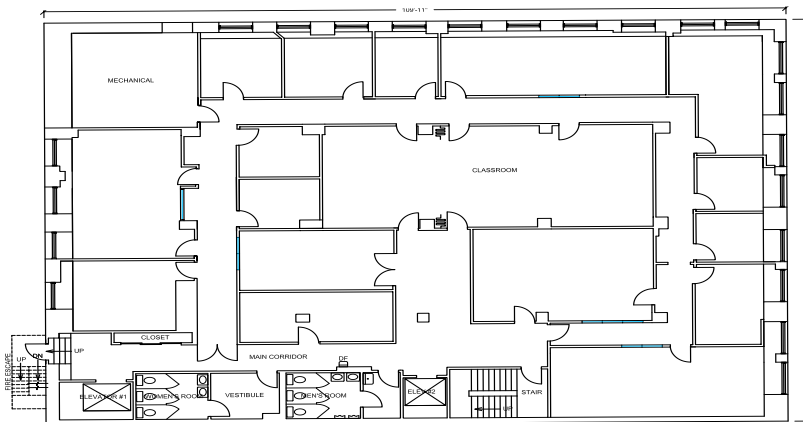
FIFTH FLOOR PLAN
